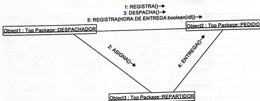
Fig. 4. Communication Diagram from PS in the Figure 2.
