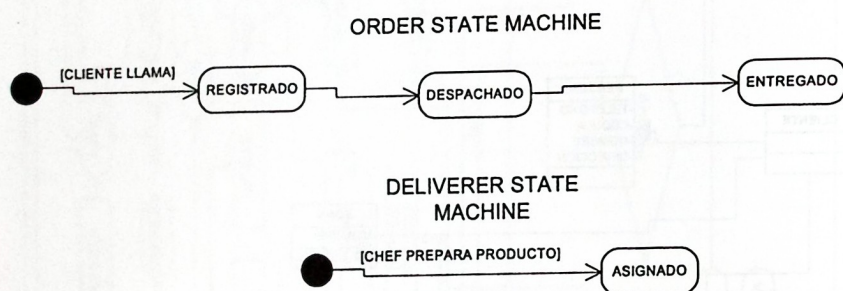
Fig. 5. Resultant State Machine Diagrams from PS in the Figure 2.
